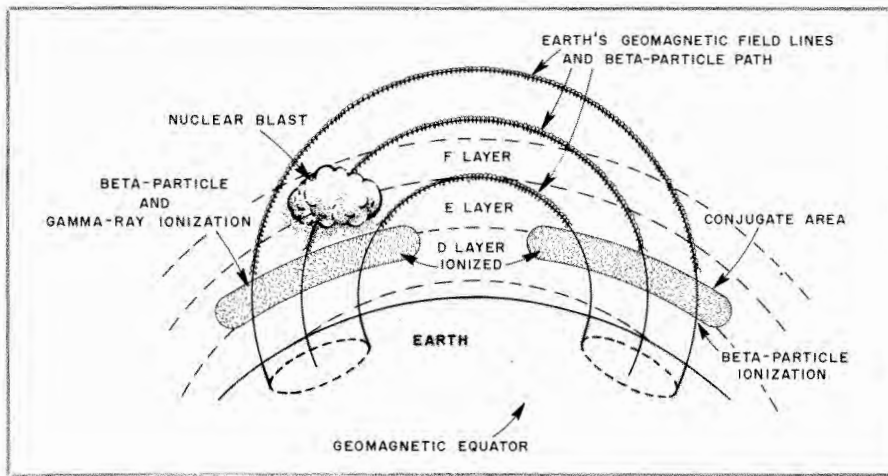
Fig 3—Depiction of the magnetic conjugate.
